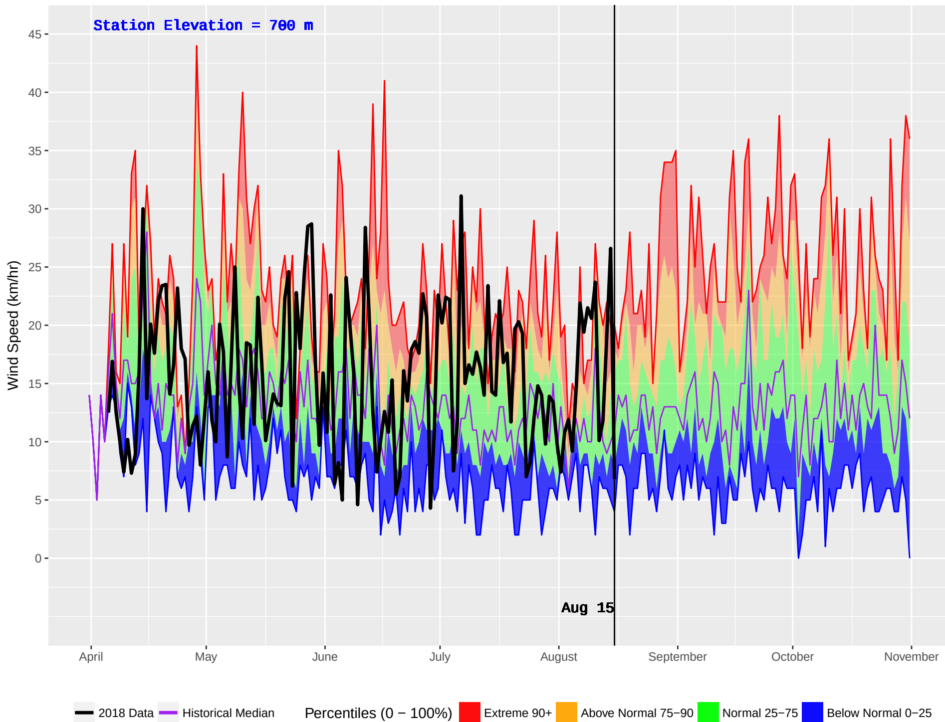
OSBORN (1045) : Historical (2009–2016) and Current (2018) Daily Wind Speed
