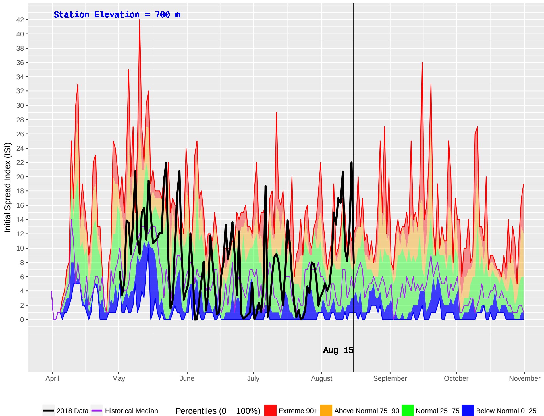
OSBORN (1045) : Historical (2009–2016) and Current (2018) Daily Initial Spread Index (ISI)
