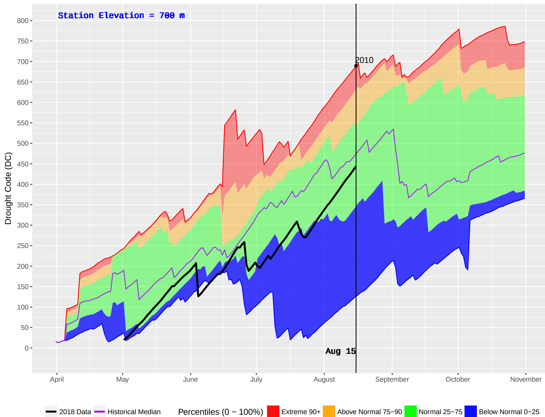
OSBORN (1045) : Historical (2009–2016) and Current (2018) Daily Drought Code (DC)
