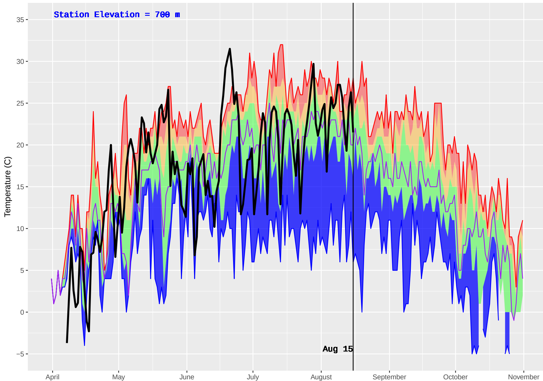
OSBORN (1045) : Historical (2009–2016) and Current (2018) Daily Temperature
