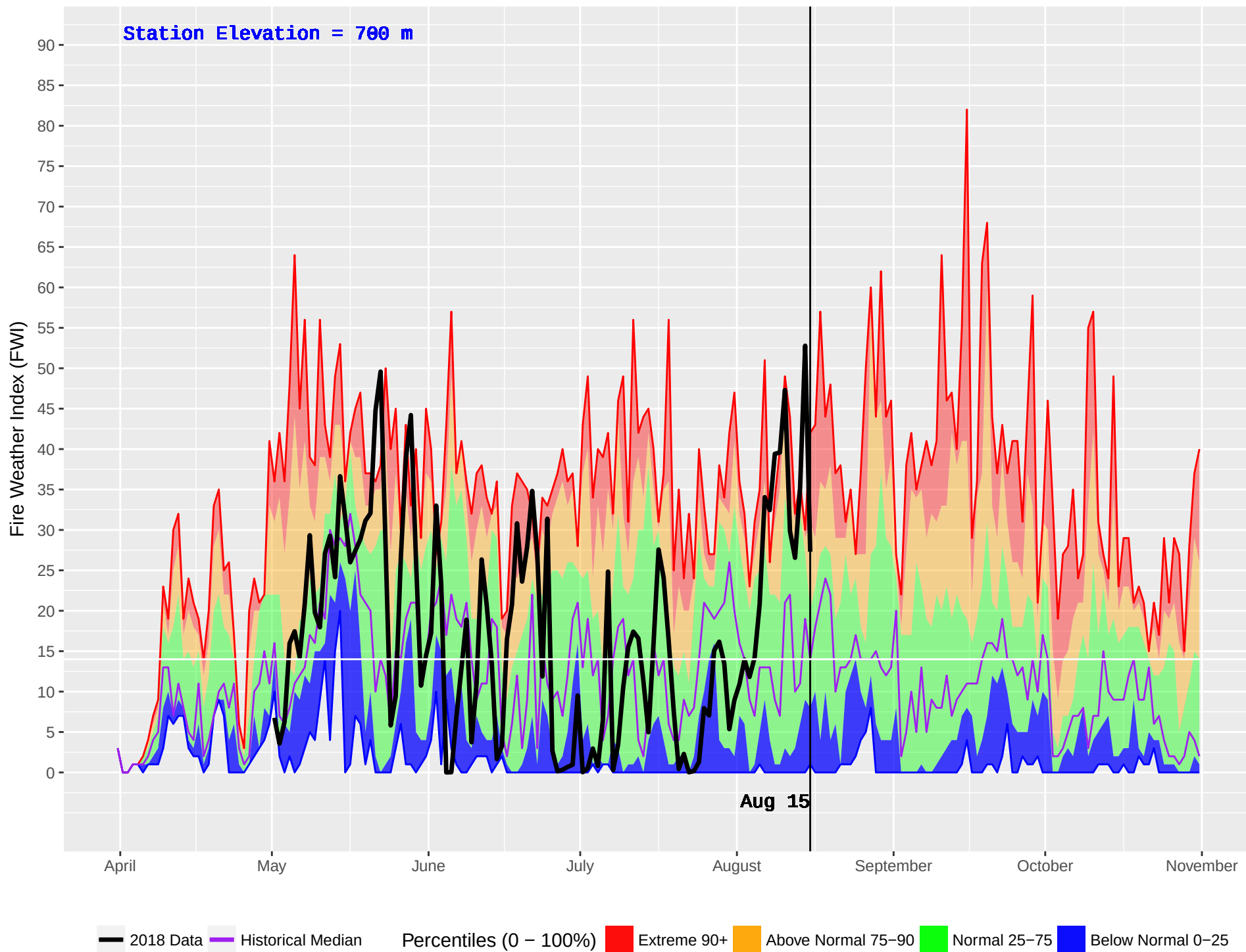
OSBORN (1045) : Historical (2009–2016) and Current (2018) Daily Fire Weather Index (FWI)
